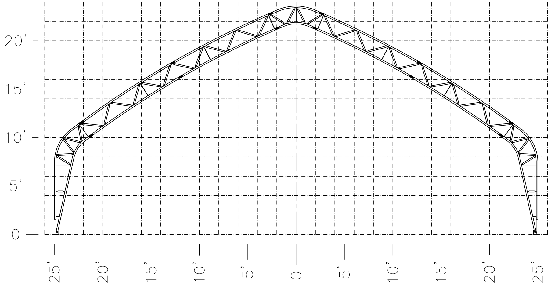
50' MBS GRID = 2' x 2'
