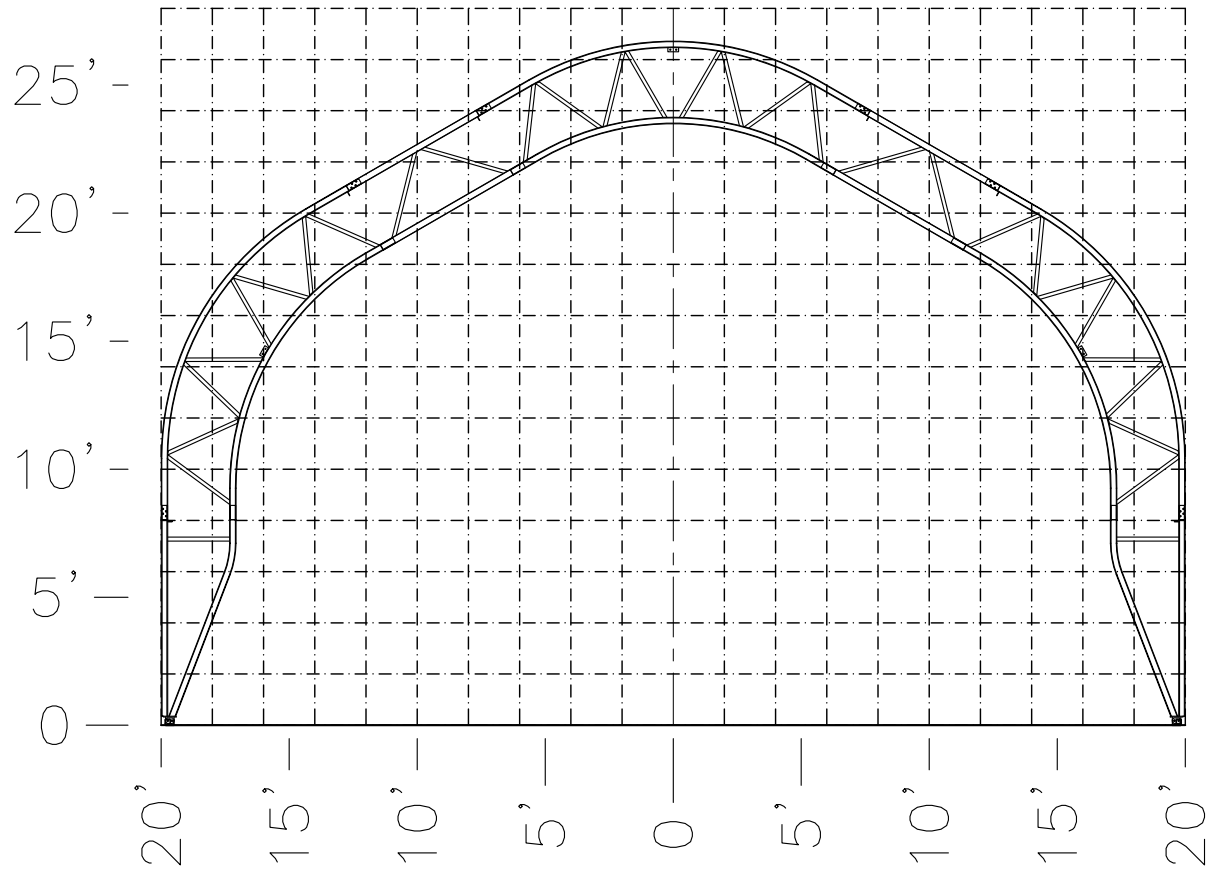
40' TBS2 □ GRID = 2' x 2'
