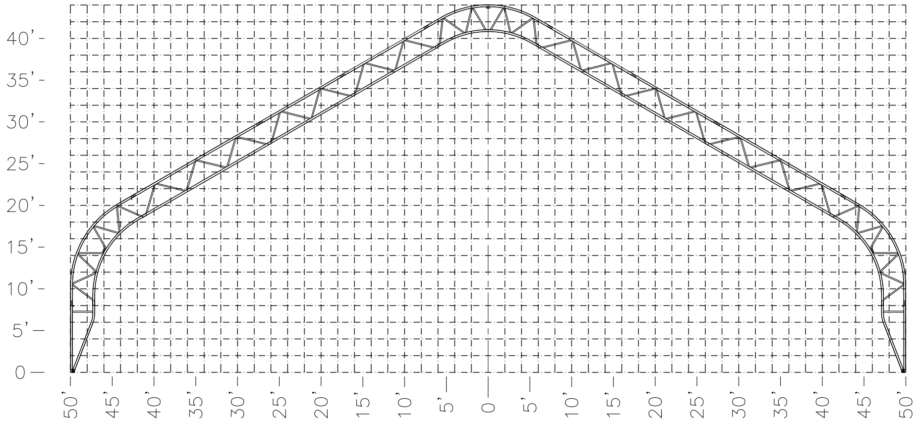
100' TBS2 □ GRID = 2' x 2'
